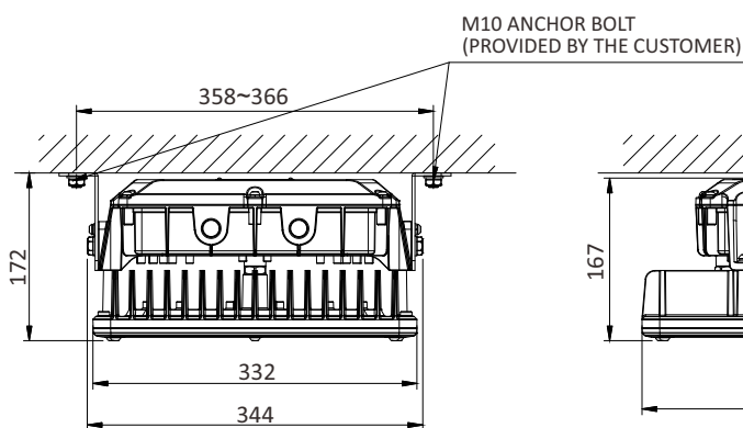
BR-SEB-G Ceiling mount
