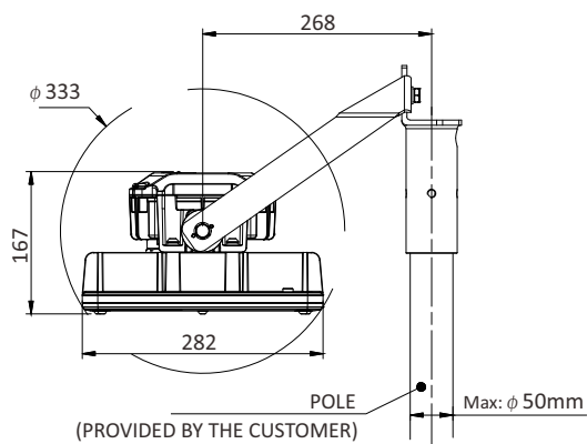
SBT-SEB-G+SBT2-F-G Pole Mount
