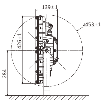
SBT-TK-4-G Four lamps
