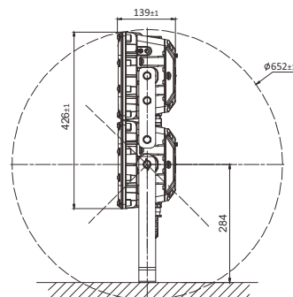
SBT-TK-4-G Four lamps
